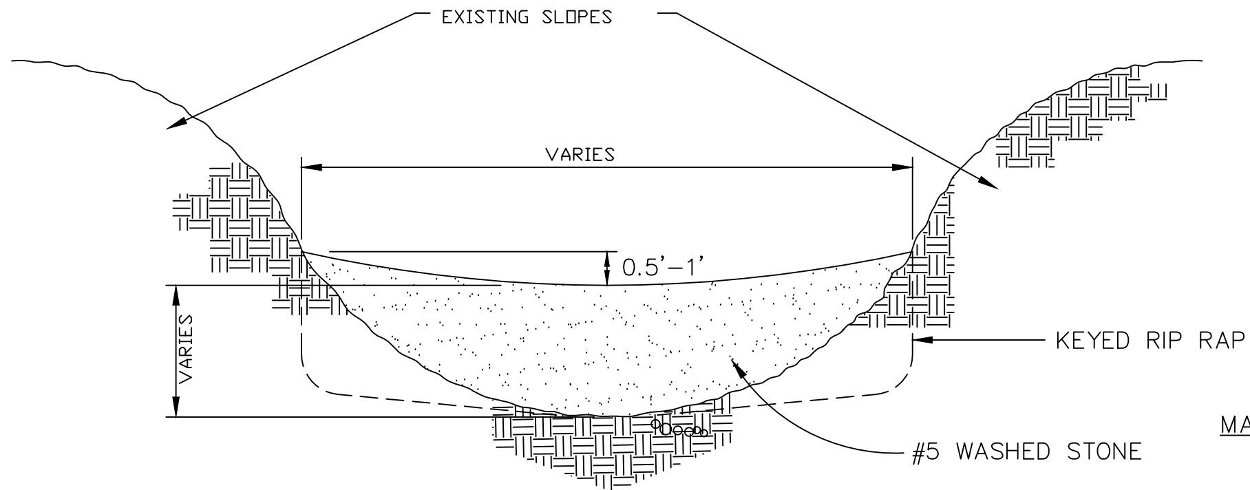
FRONT VIEW
