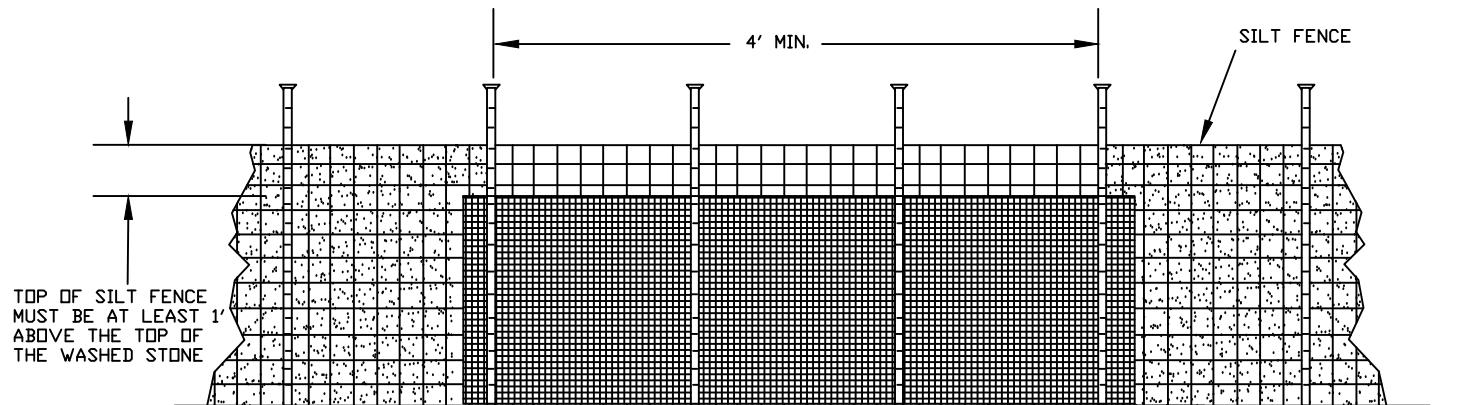
FRONT VIEW
