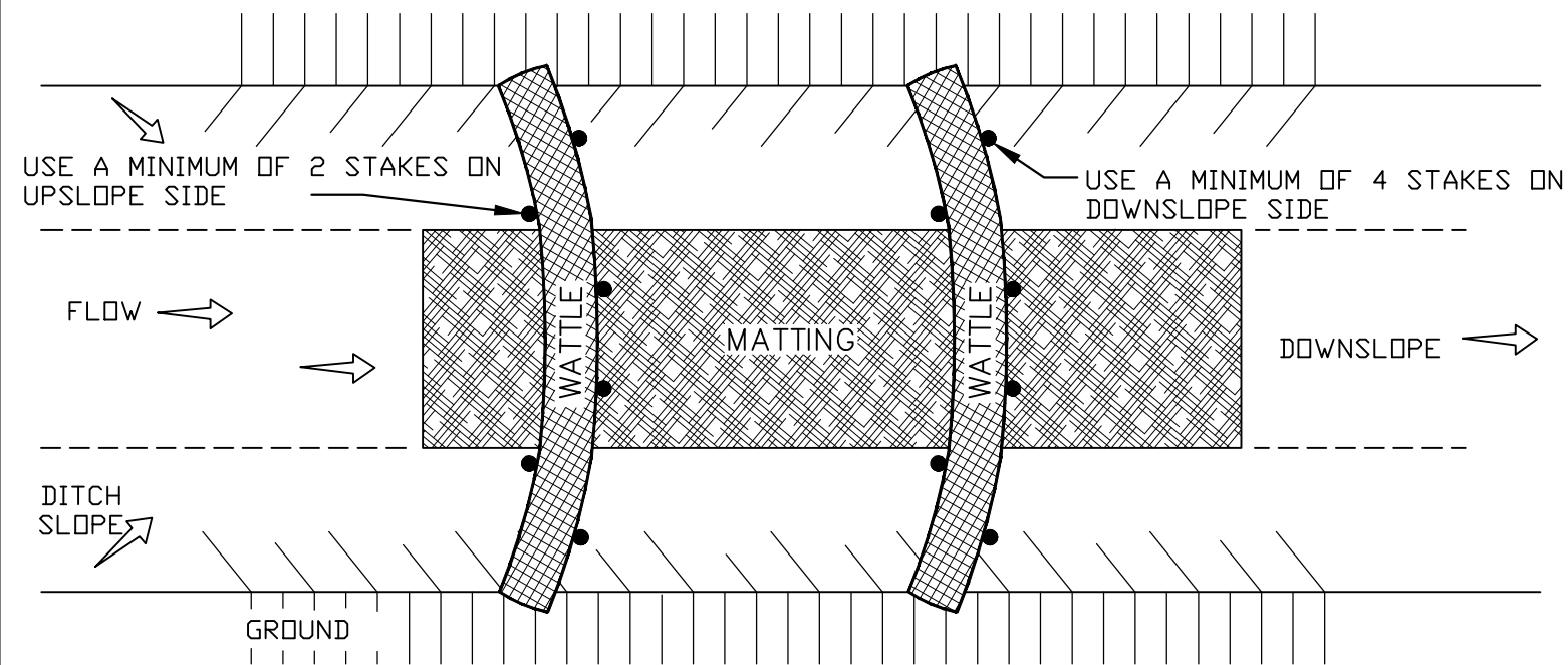
PLAN VIEW
