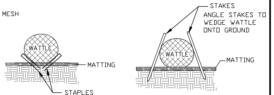
STAPLE INSTALLMENT SECTIONS
